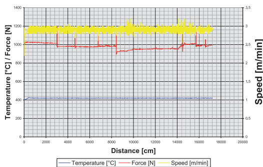
Graphical evaluation of a weld seam (Length: 560 ft)
