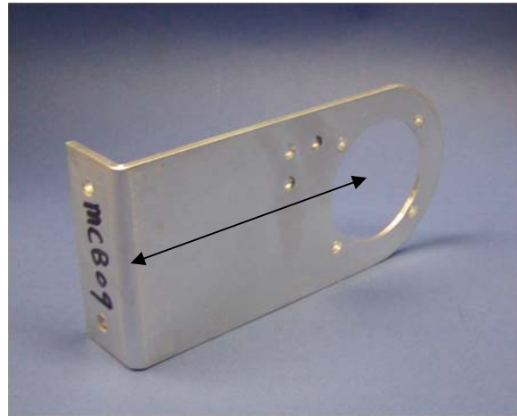
Distance from the center of the bracket hole To the bottom of the bracket is 116mm
