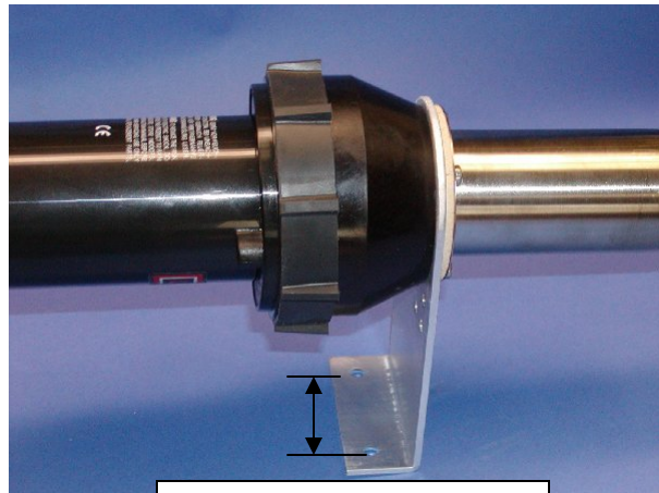
53 mm between hole centers. Bolt holes 6 mm in diameter.
